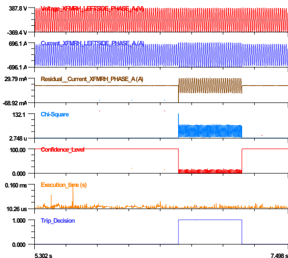
Figure 8: 5% Internal Turn-Ground Fault of Transformer
