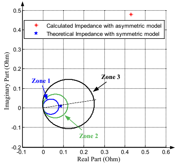
Figure 5. Distance Relay Characteristics
