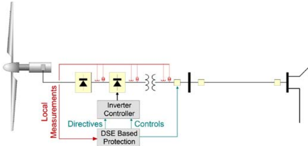
Figure 9: Example of CIG Integrated Protection and Control
