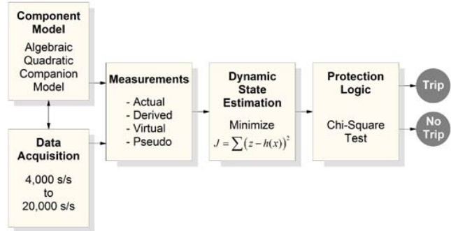
Figure 2: Dynamic State Estimation Based Protection Method
