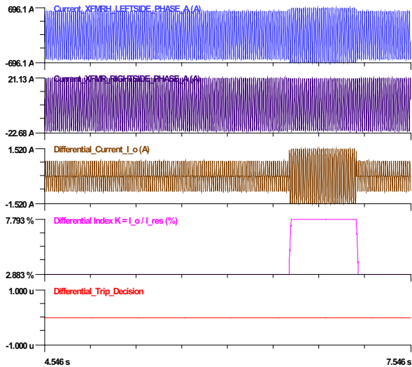
Figure 7: Results of the Differential Protection Scheme
