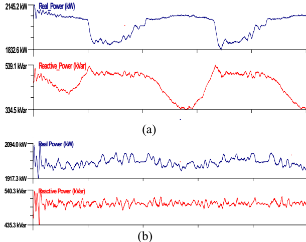
Figure 10: Inverter Real and Reactive Power during a Disturbance Without Integrated Protection & Control (a), with proposed system (b)
