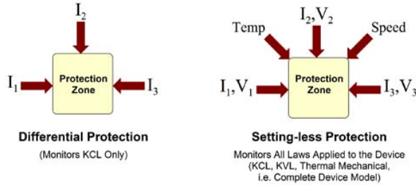
Figure 1: Evolution of the Differential Protection Function [15]
