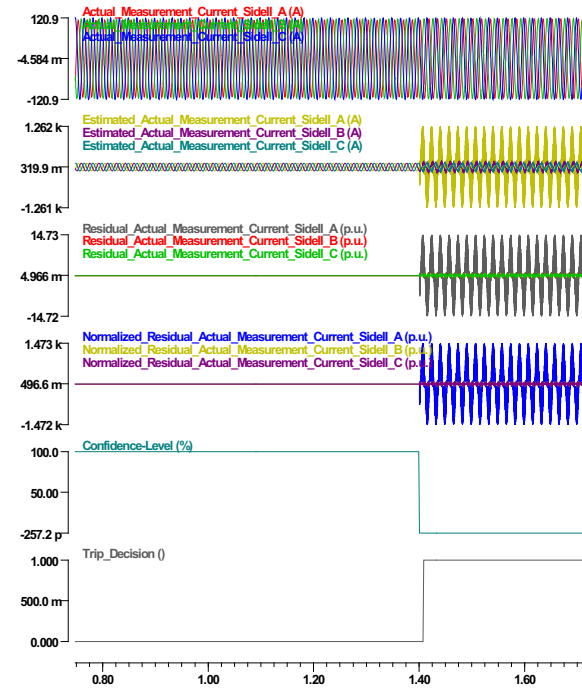
Figure 6. Phase A-N Internal Fault at 1.4s
